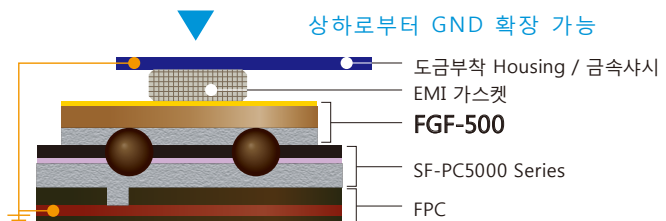
FPC+Shield Film
